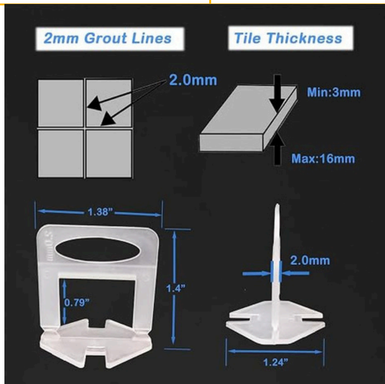
Tile Spacer Wedges System
